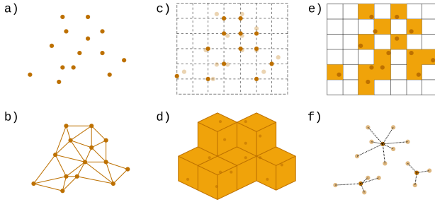
Figure 3. Illustration of various point cloud representations: a) raw points, b) mesh, c) grid rounded, d) voxel, e) raster, f) skeleton.
